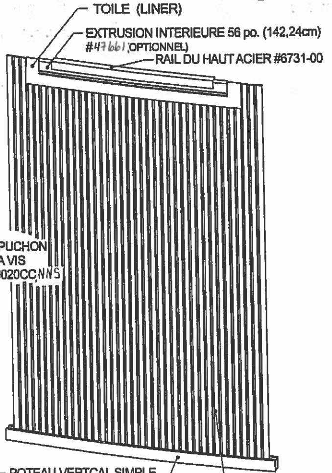
POTEAU VERTICAL SIMPLE ACIER #7720SP52(54)R4
